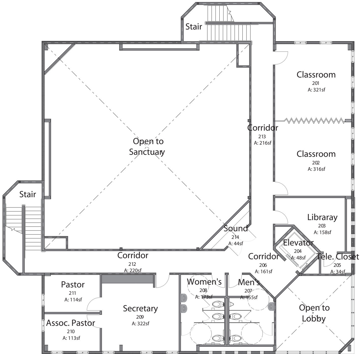
Genesis 5 Floor Plan Second Floor Reduced Scale
